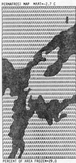
Figure 3. Simulated effects of different mean annual air temperatures on permafrost distribution.
