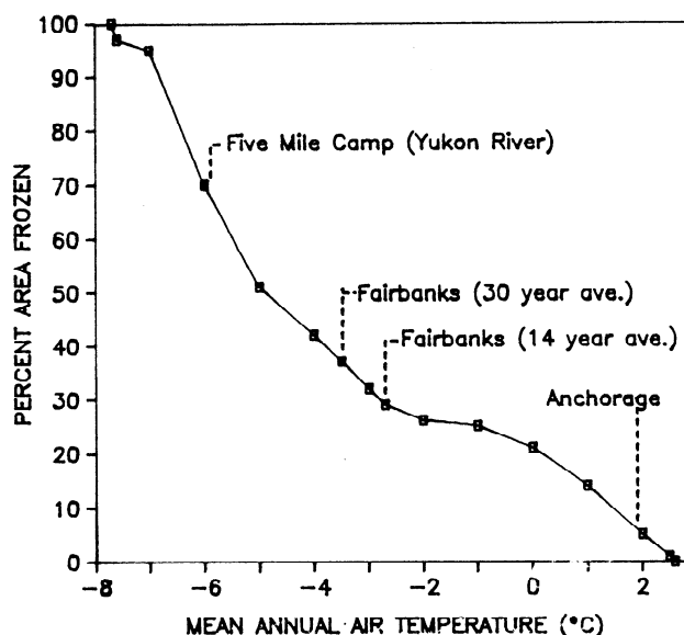
Figure 4. Simulated effects of changes in mean annual air temperatures on the percent of area frozen. Air temperatures at Five Mile Camp and Anchorage are included for comparison.
