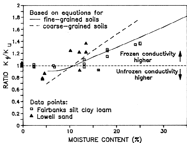
Figure 1. Effects of soil moisture on the ratio of frozen ( K_f ) to unfrozen ( K_u ) thermal conductivities. Ratios of equations (5)/(4) and (7)/(6) are plotted (see text). Data and equations are from Kersten (1949).
