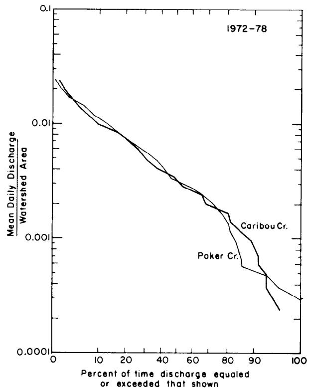
Figure 20. Flow-duration curves of the mean daily discharge per watershed area for Caribou and Poker creeks, 1972-1978.
