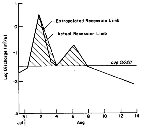
Figure 12. Method of calculating storm discharge.
