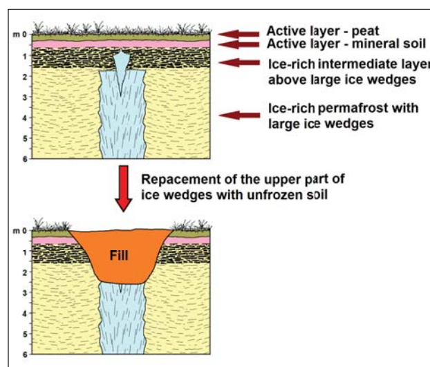
Figure 6. For new construction, removing the upper portion of ice wedges and replacing the ice with fine-grained thaw stable soils will protect ice wedges from degradation and reduce thermal erosion and ponding beneath the buildings. (Credit: Y. Shur and M. Kanevskiy)
