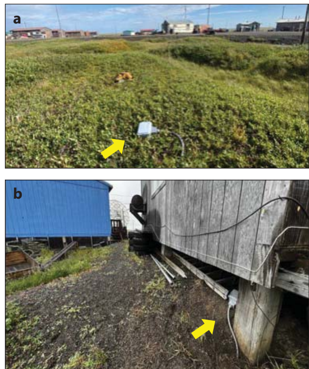
Figure 10. a. A ground temperature station installed on dry tundra in a natural site. b. A ground temperature station located on a foundation pile on a house without skirting. (Credits: D. Nicolsky)
